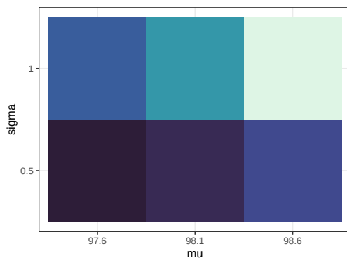
(a) Prior distribution.
